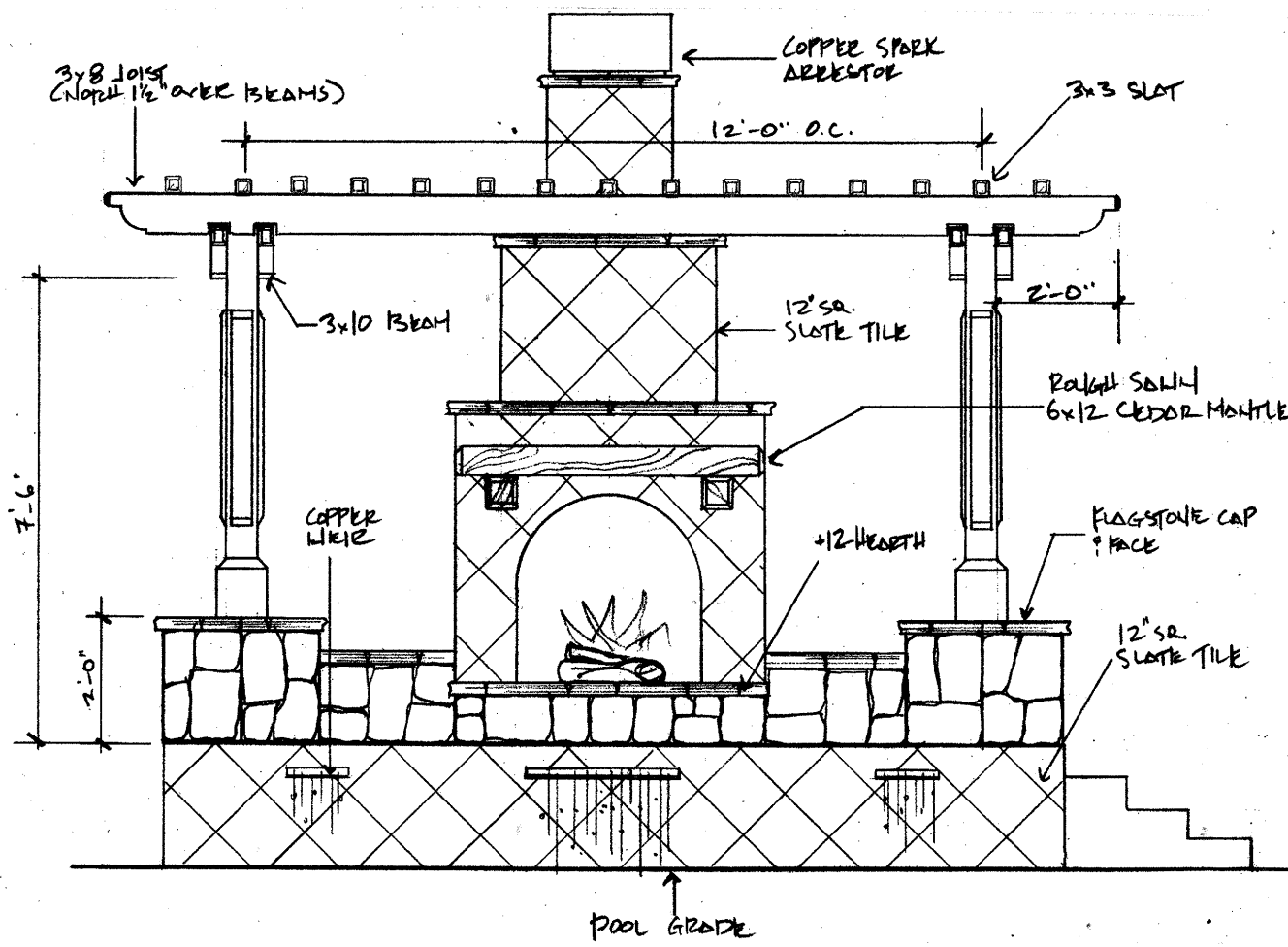
A FIREPLACE PATIO AT POOL - FRONT ELEVATION SCALE: 1/2" = 1'-0"
